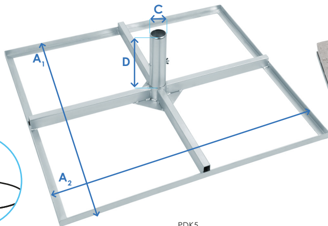
PDK5
