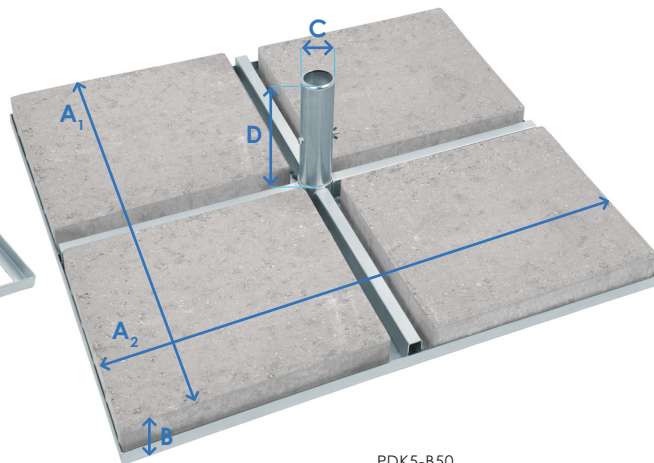
PDK5-B50
