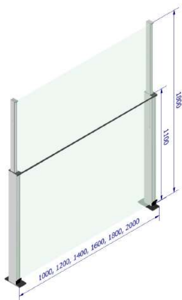
Wind Barrier
